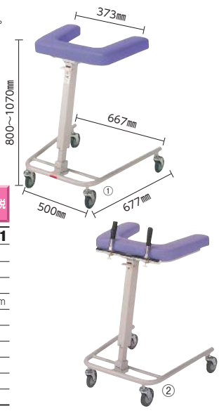
Rollator
